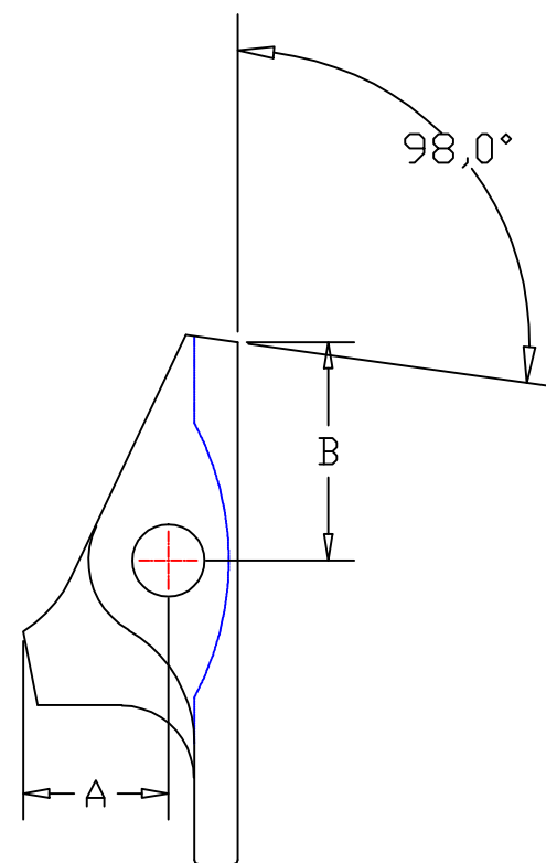
Milled Magazine Catch Drawing 3-22110_56-A-212_0-11
