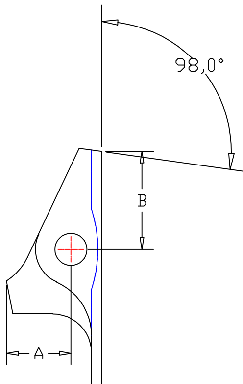
Stamped Magazine Catch Drawing 2-24344_BП1_0-11
